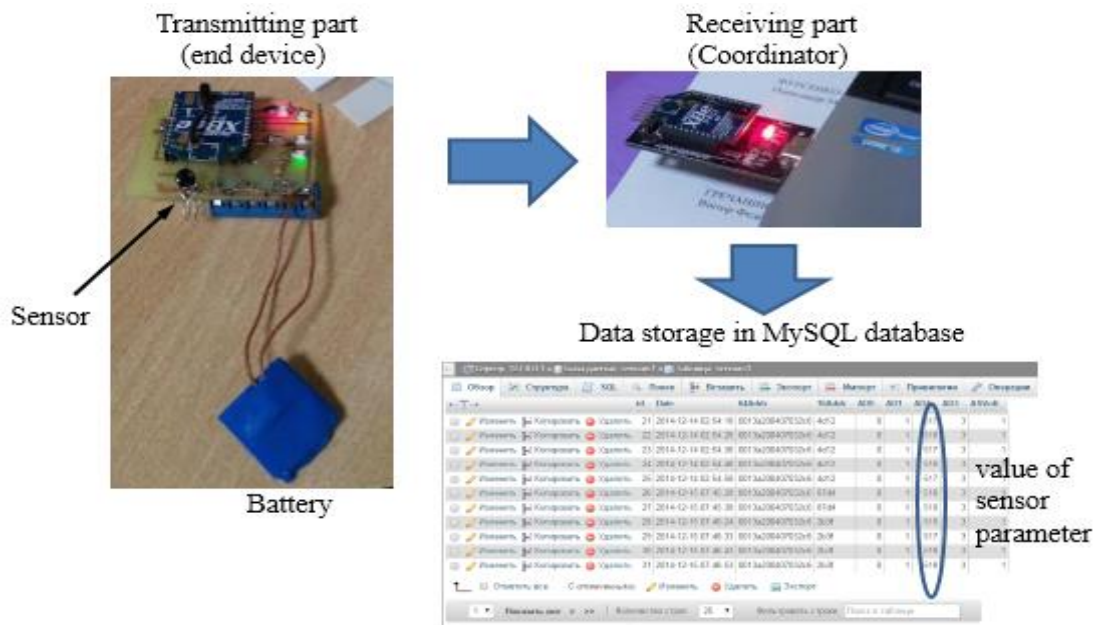
Picture 4 WSN model based XBee radio modules
