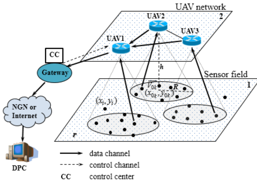
Picture 2 Example of WSN architecture using UAVs
